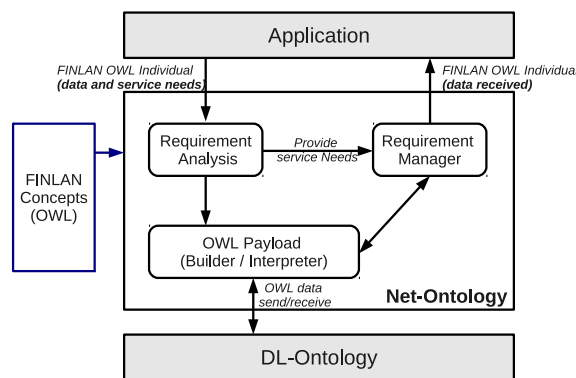
Figure 1. Net-Ontology modules.
