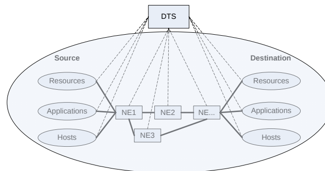
Figure 1 – DTS Topology
